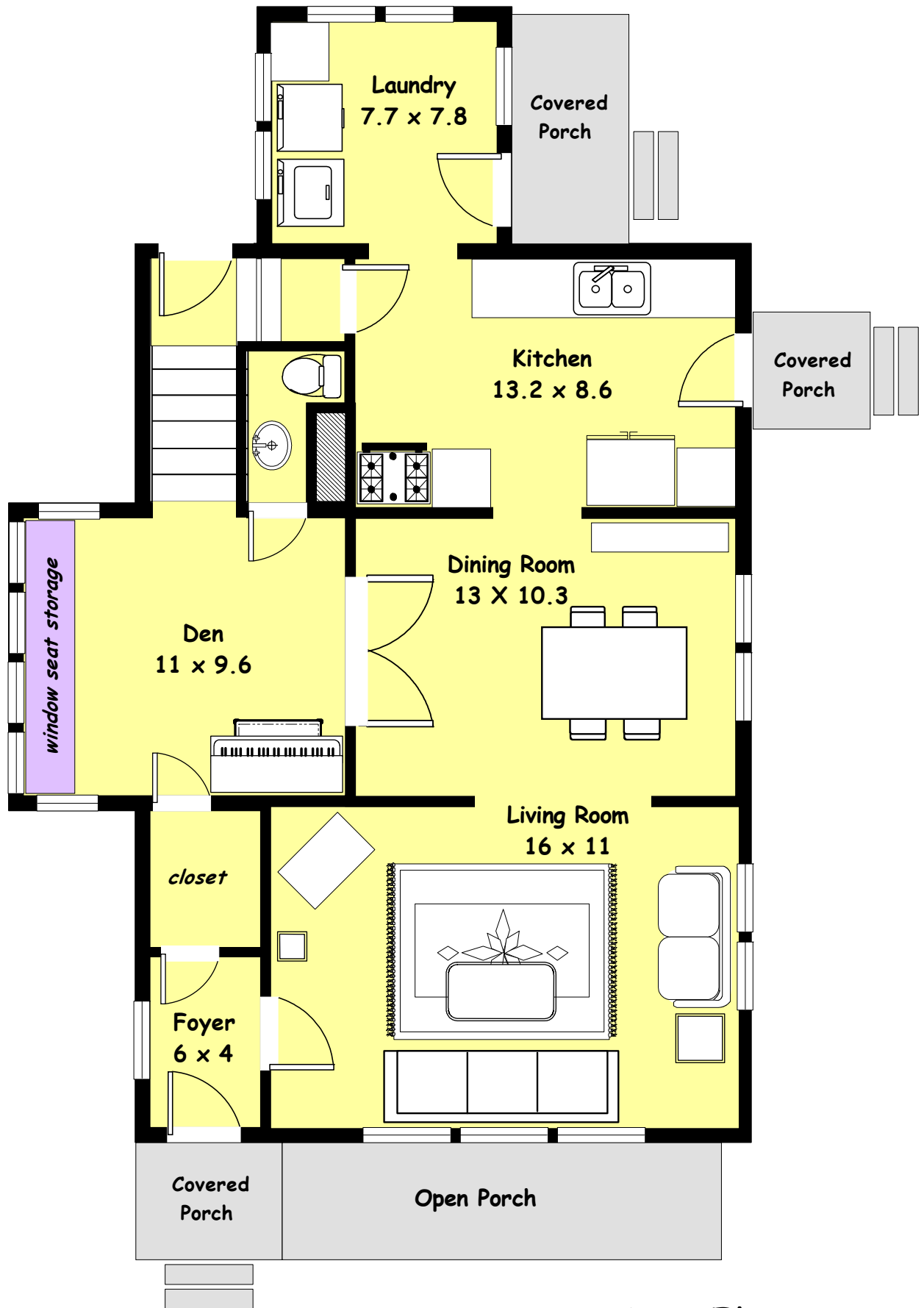
Main Floor 734 square feet
